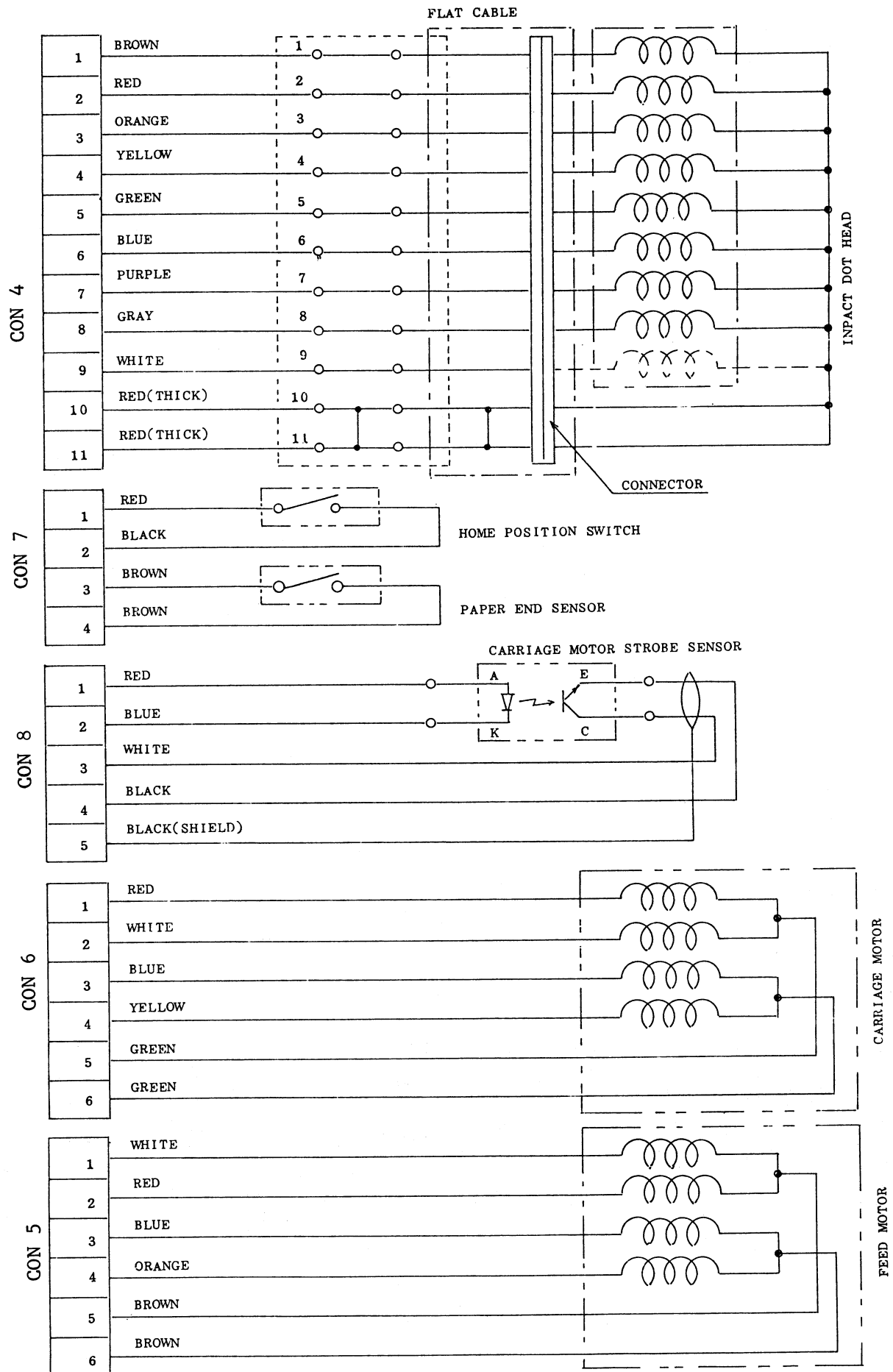
Figure 22. Connection Diagram
