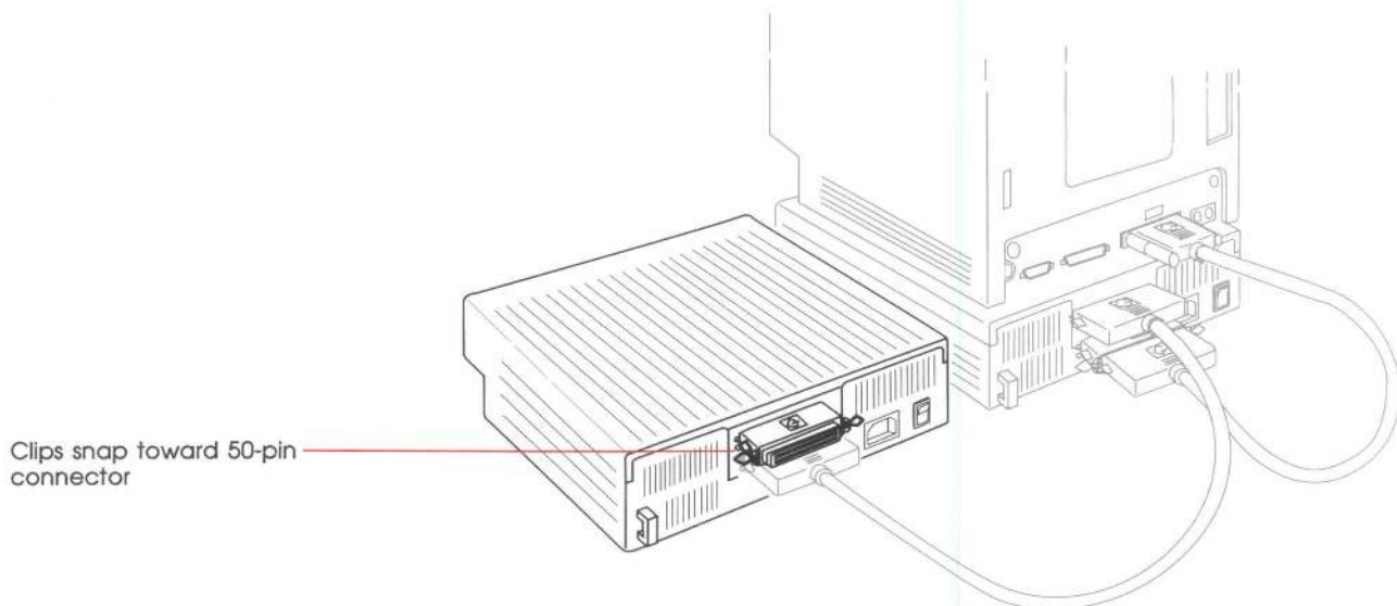
Figure 1-15 Attaching the Cable Terminator to the Tape Backup 40SC
