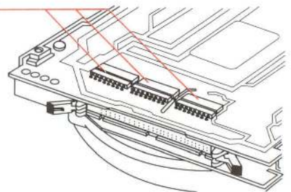
Figure 1-9 Terminating resistors
