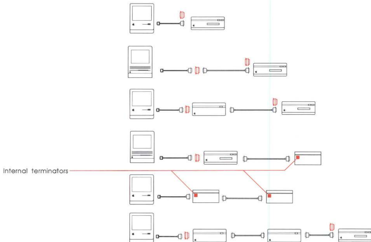
Figure 1-10 Macintosh computers without an internal hard disk and external SCSI devices
