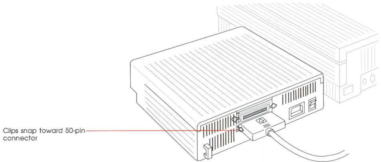
Figure 1-21 Attaching the System Cable to the Tape Backup 40SC
