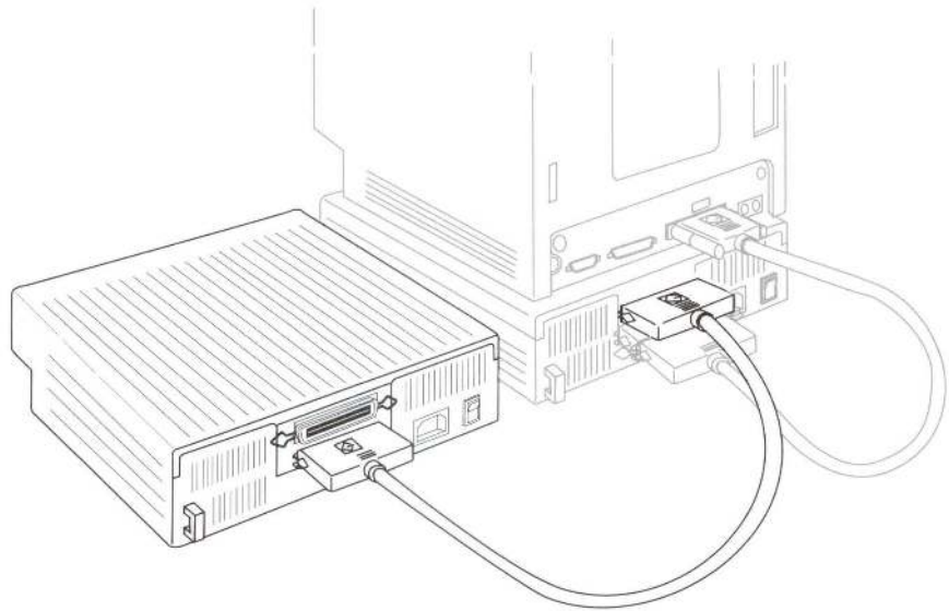
Figure 1-14 Attaching the Peripheral Interface Cable to the Tape Backup 40SC
