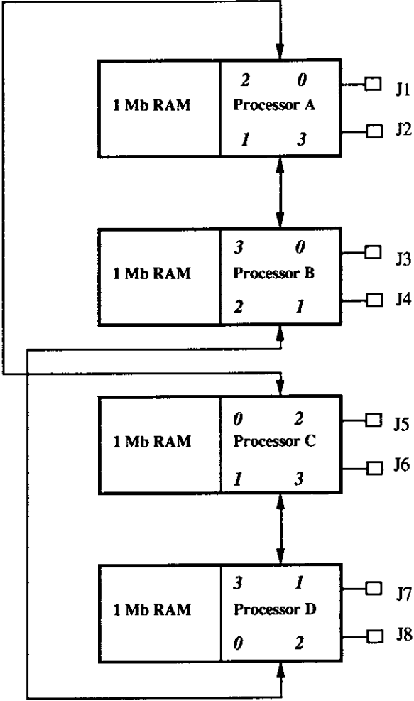
Link connection block diagram (4-processor cards)
