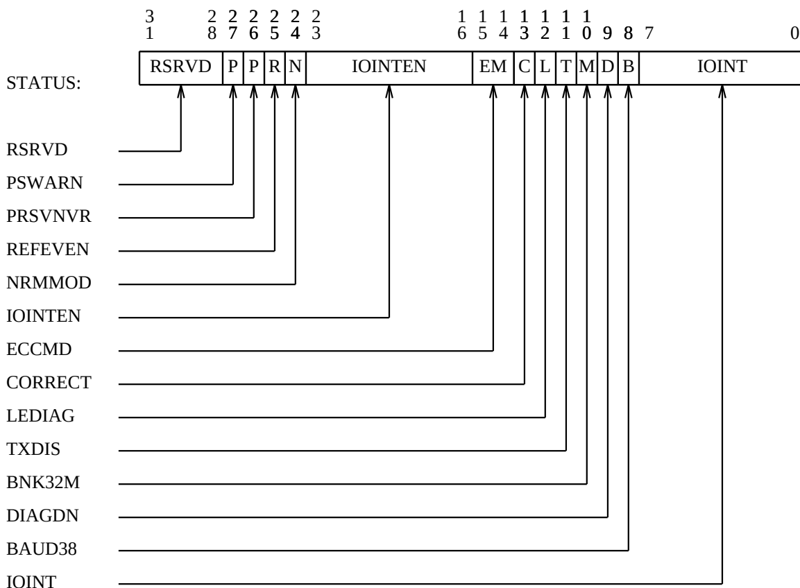
Figure 4-1: Status Register
