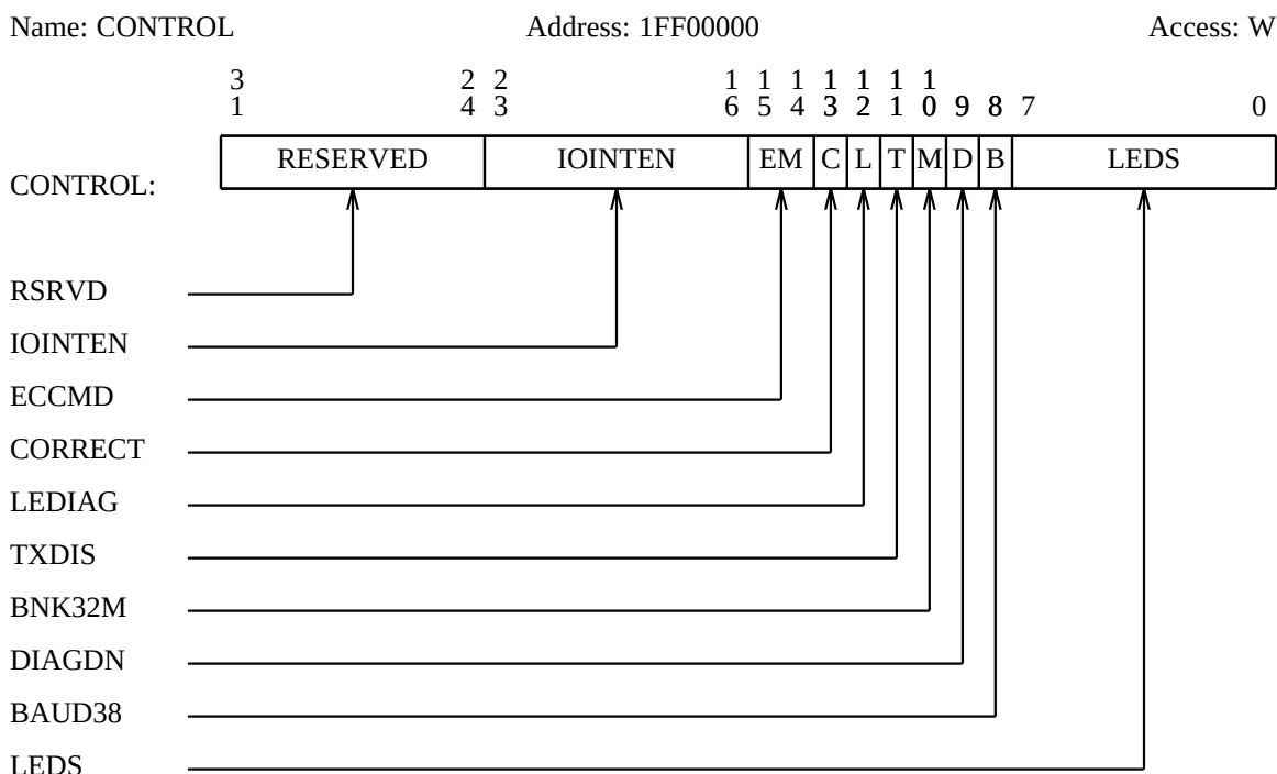
Figure 4-2: Control Register
