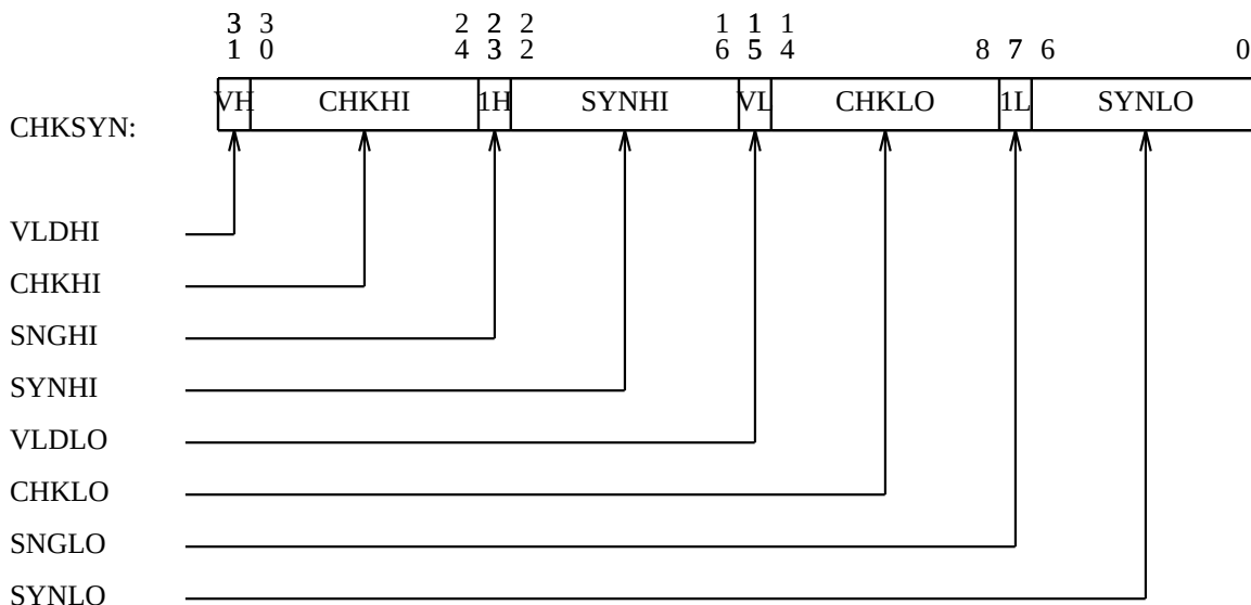
Figure 4-4: Check-bit/Syndrome Register
