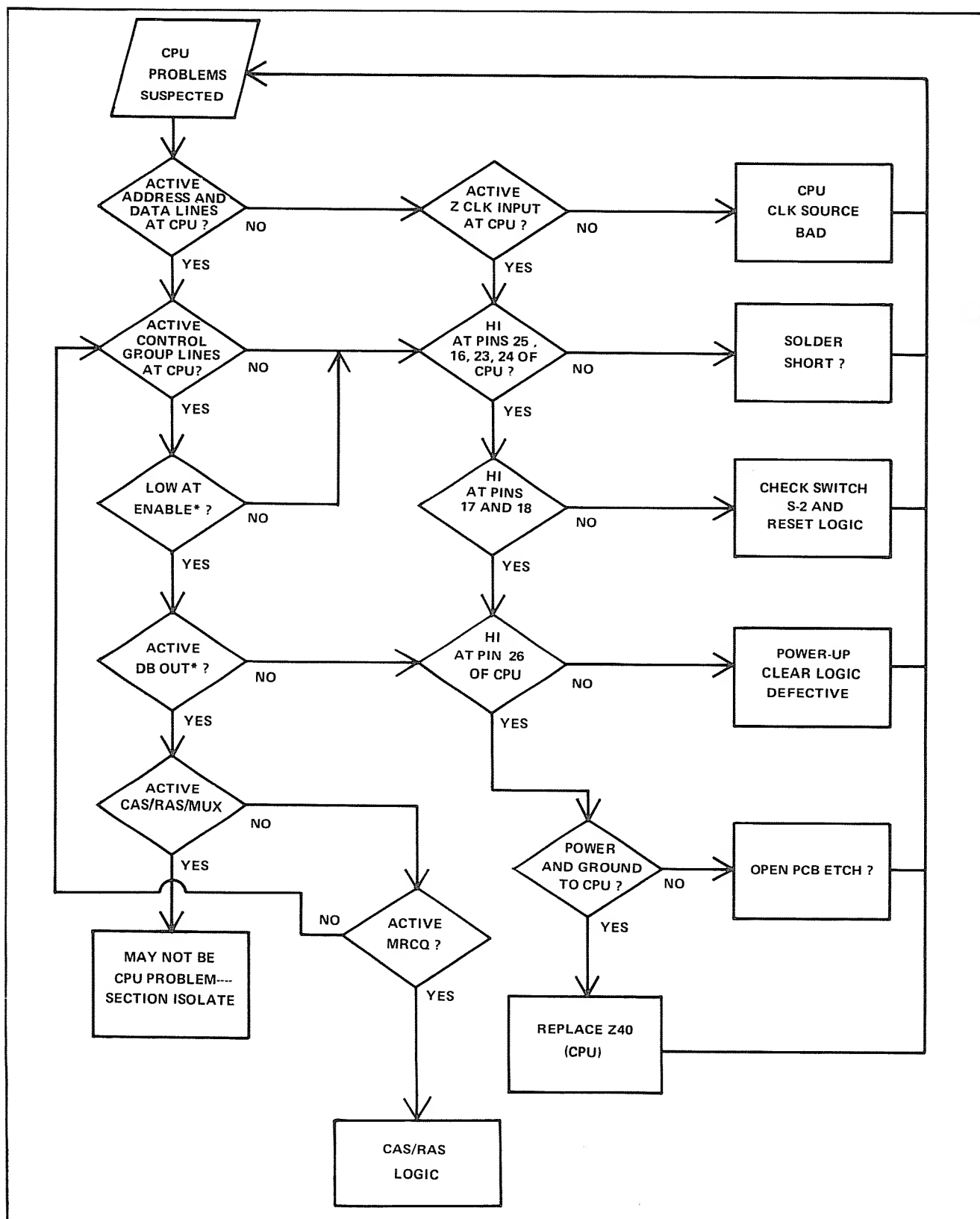
FIGURE 17. CPU Flowchart
