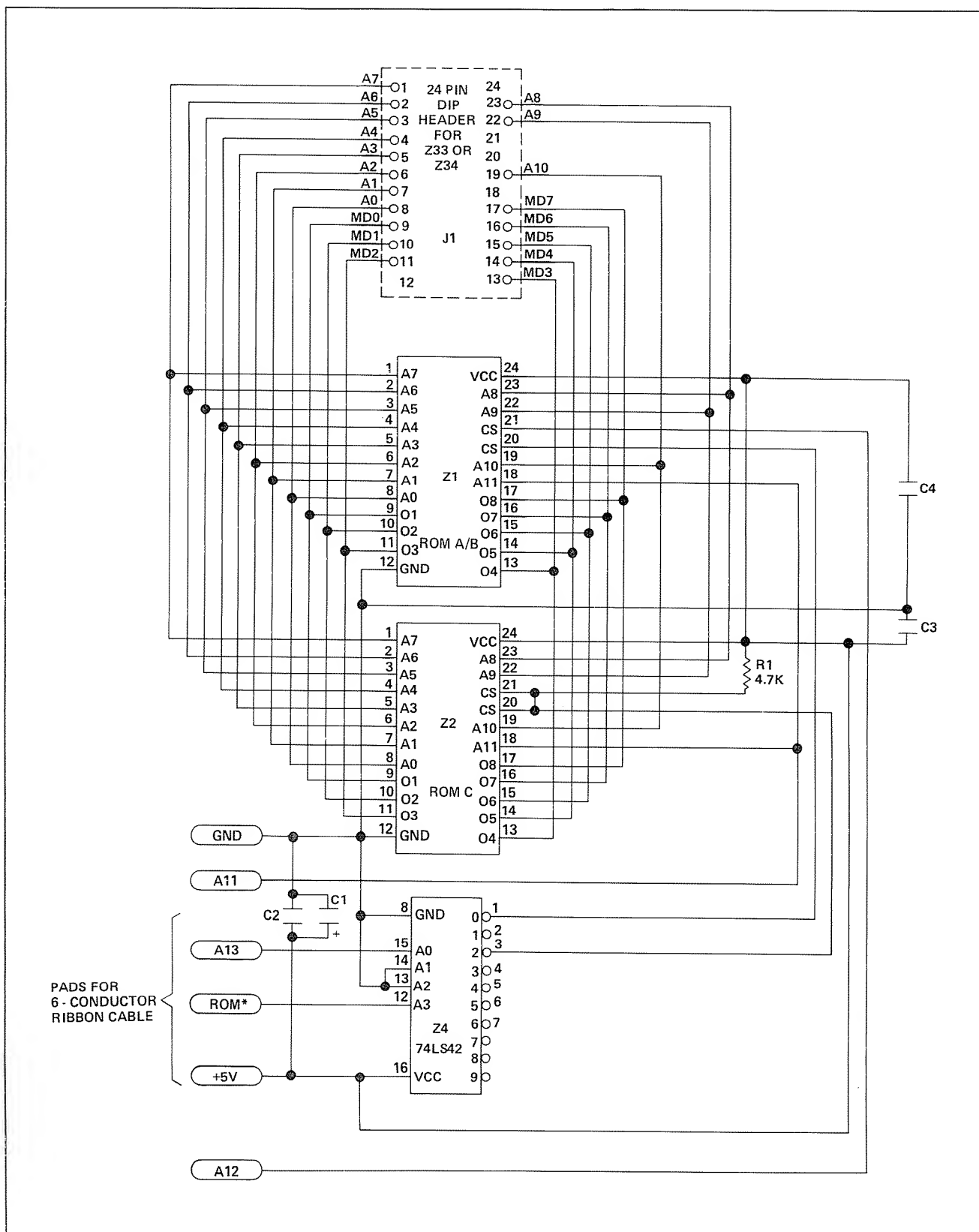
Figure 27. Level II BASIC Schematic Diagram (for CPU Boards – Current Level II ROM)
