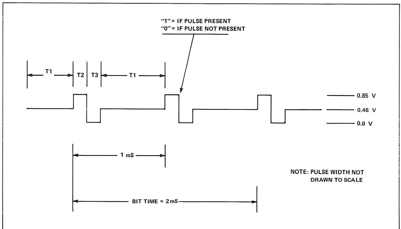
FIGURE 10. Idealized CASSOUT
