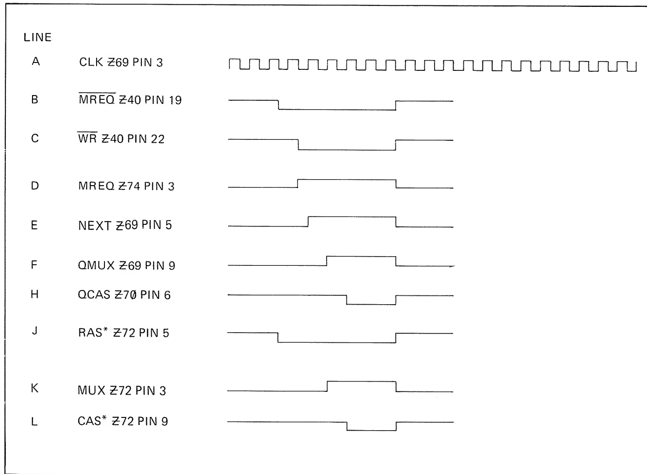
FIGURE 4. Waveform Chart
