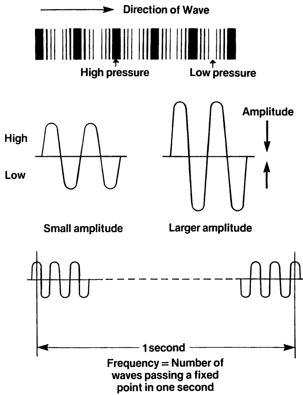
Fig. 8.2. The frequency and amplitude of a sound wave.
