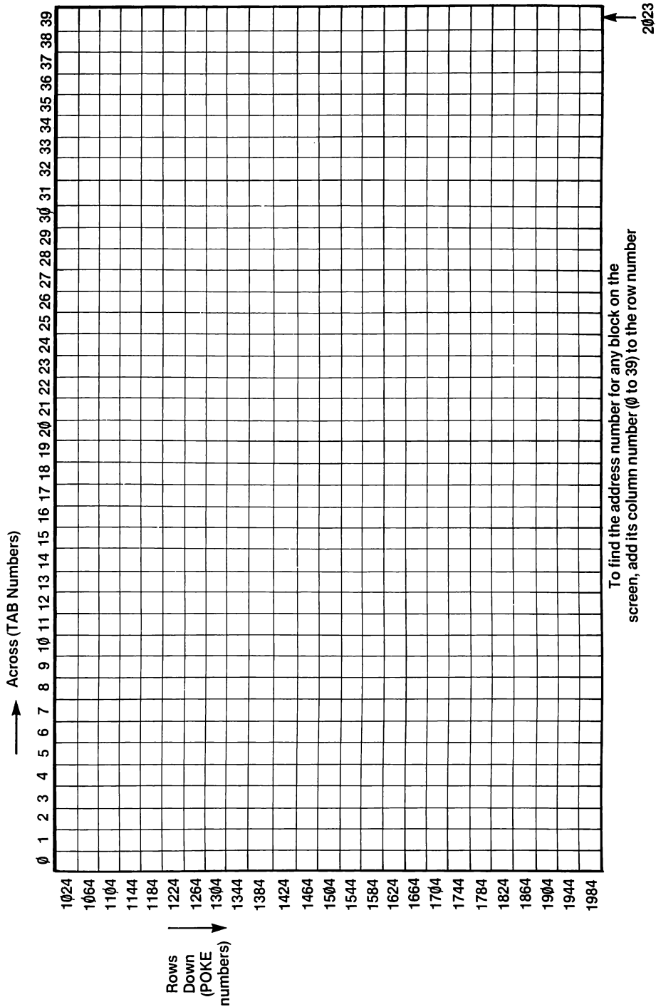
Fig. 6.7. The screen 'memory map' layout.
