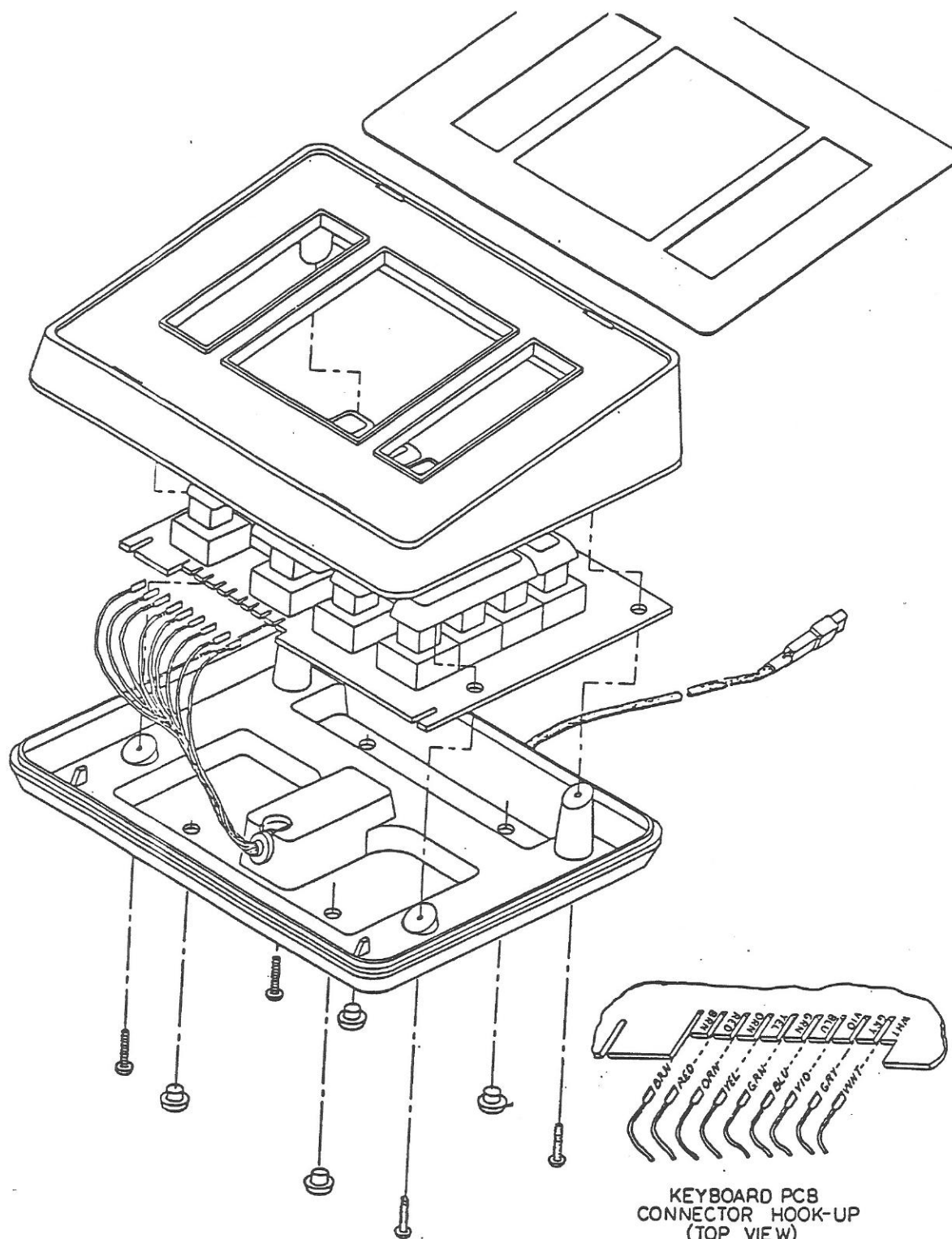
Figure 1. CX85 Assembly Drawing
