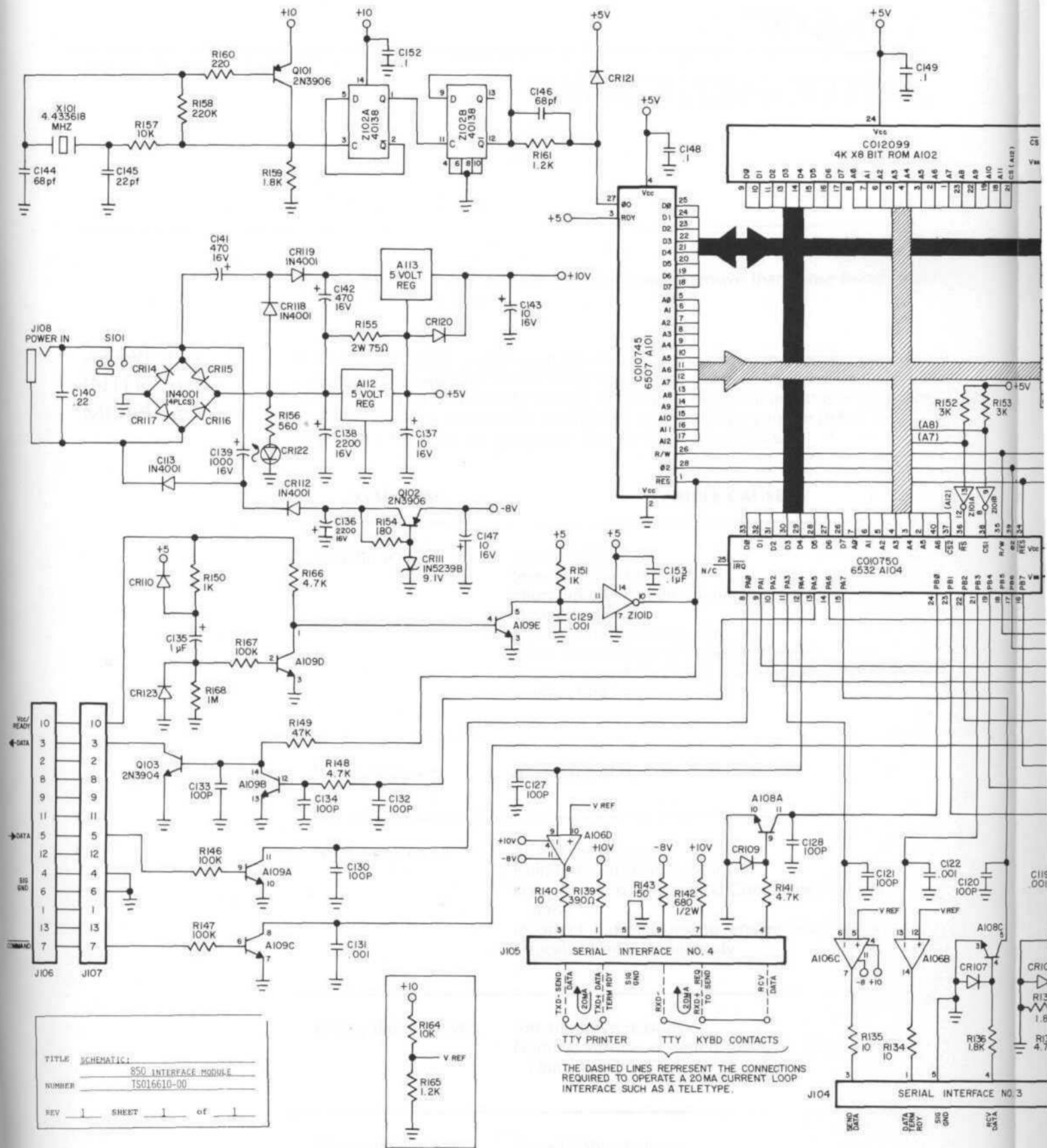
Figure C-6 Atari 850 Interface Module
